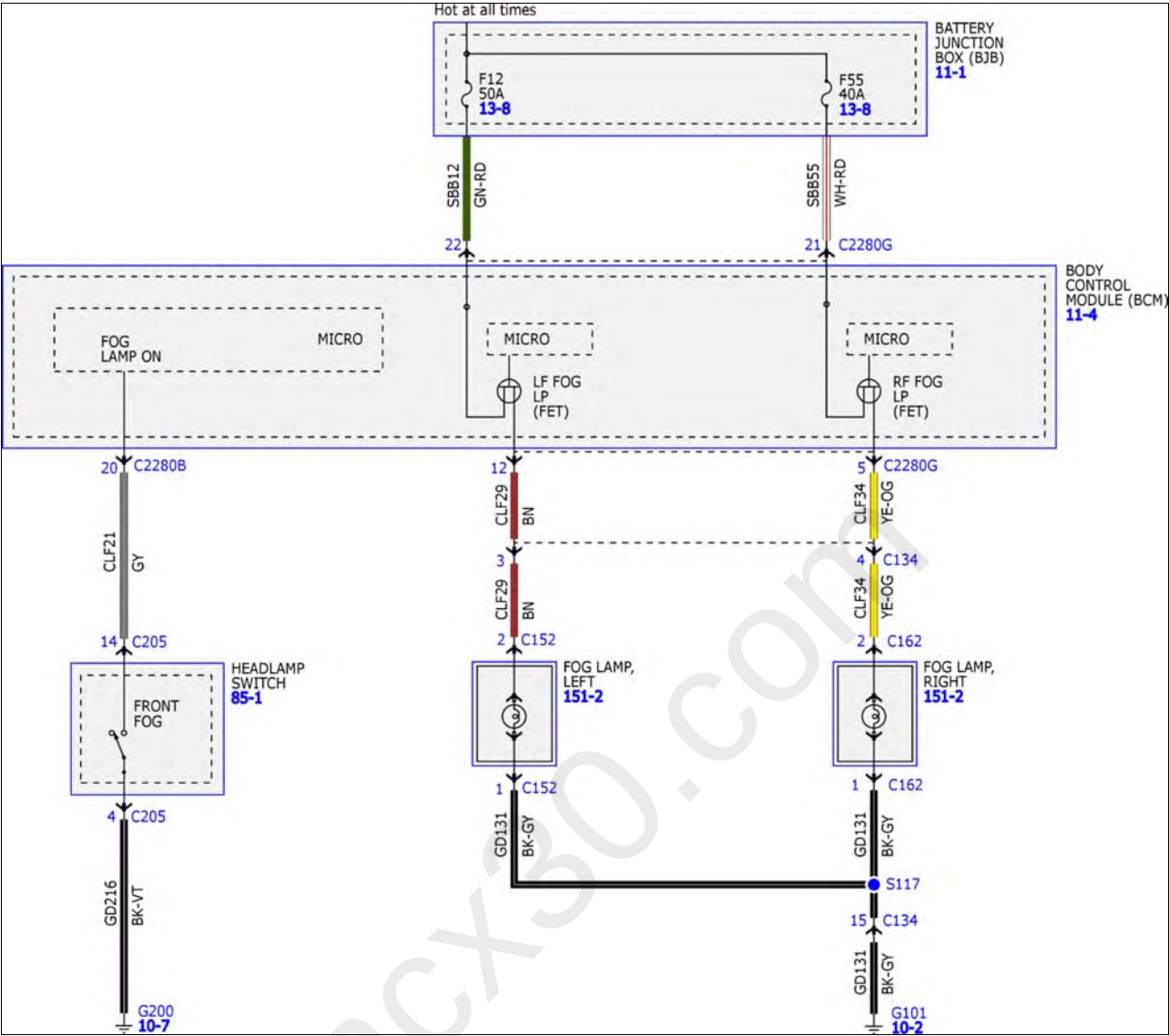
Fig 1: Fog Lamps System Wiring Diagram
